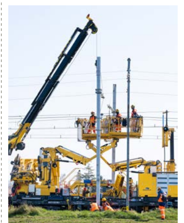
T50 train renewing overhead lines in the 1,500 volt network
